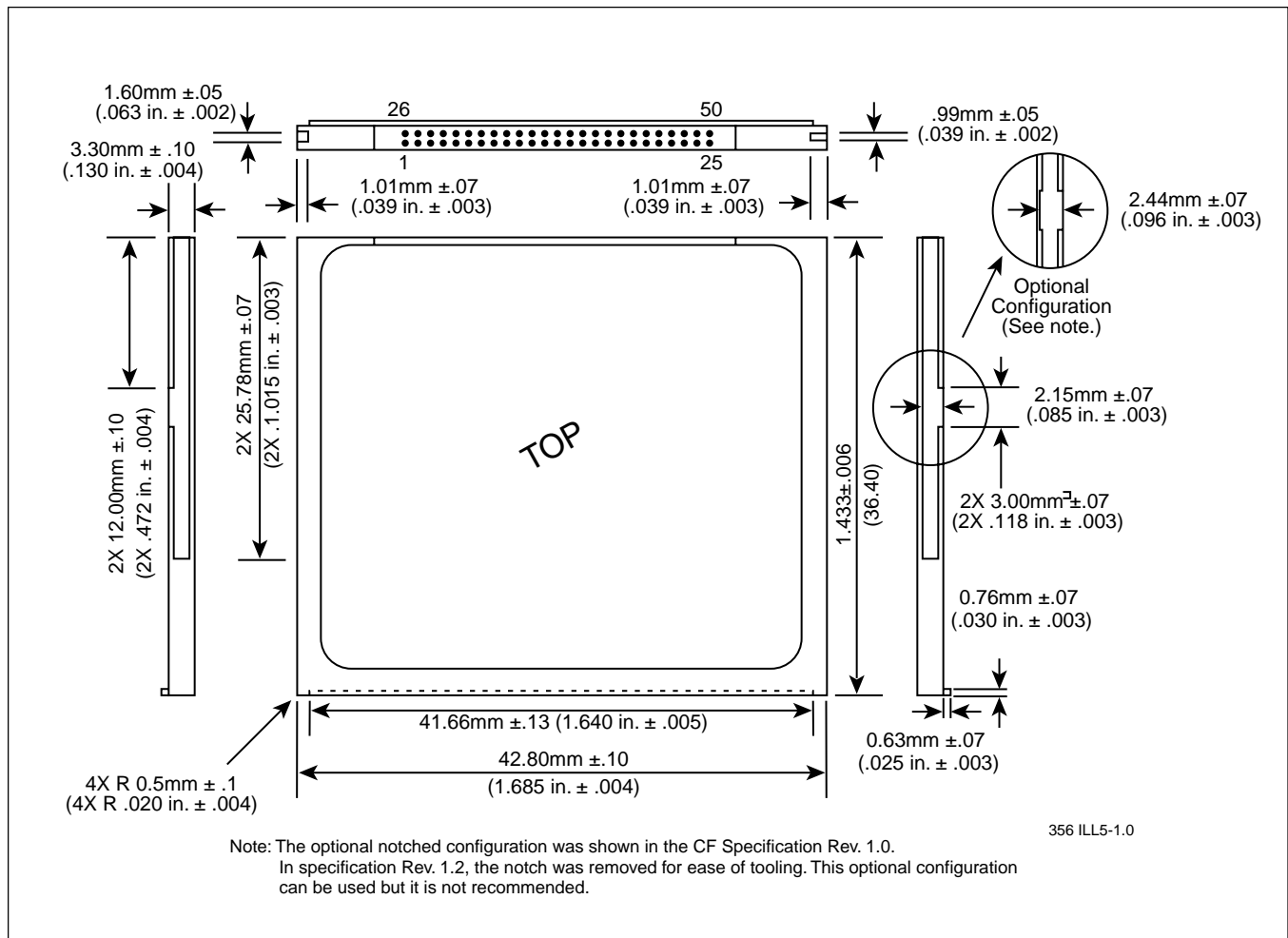
FIGURE 5-1: TYPE 1 COMPACTFLASH CARD DIMENSIONS
