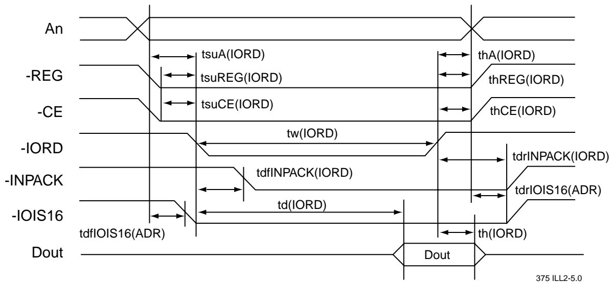
FIGURE 2-5: I/O READ TIMING DIAGRAM
