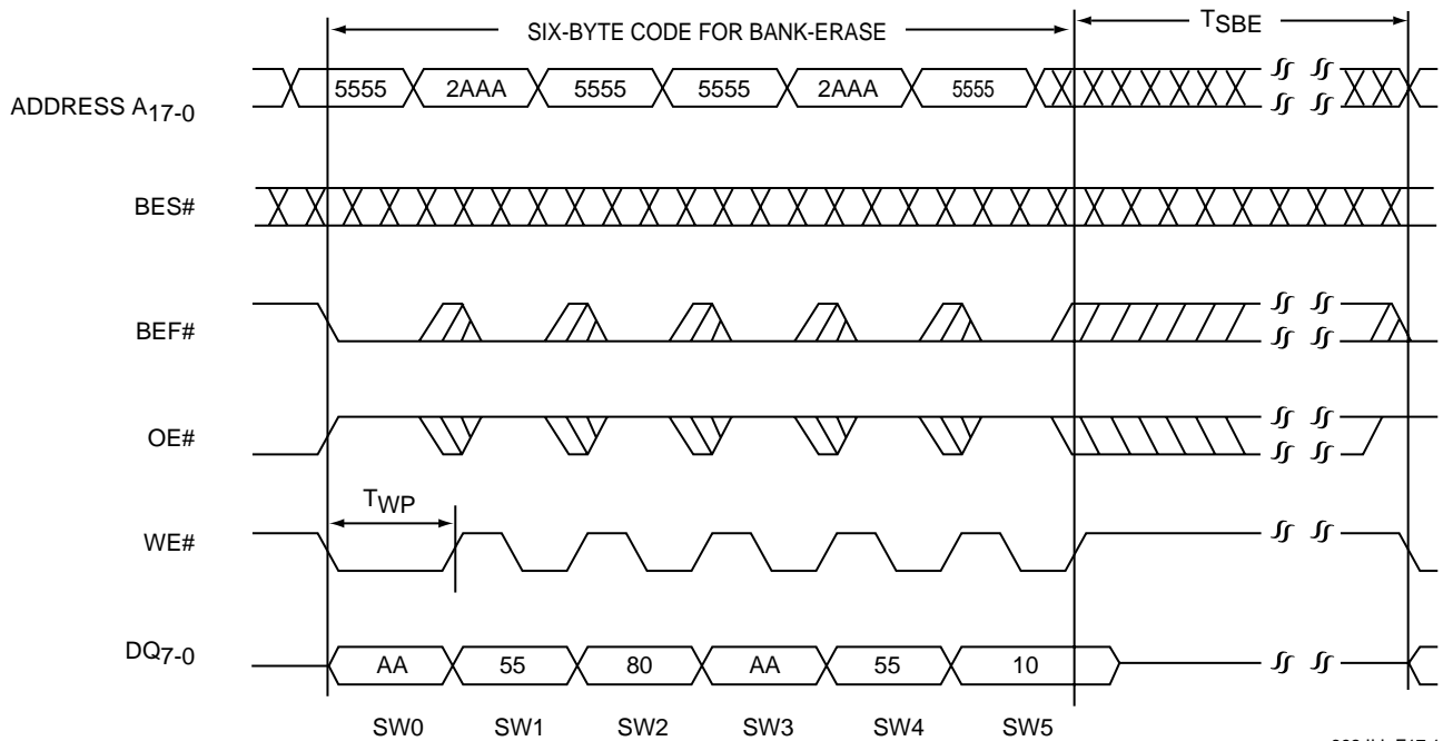
FIGURE 10: WE# CONTROLLED FLASH BANK-ERASE TIMING DIAGRAM
