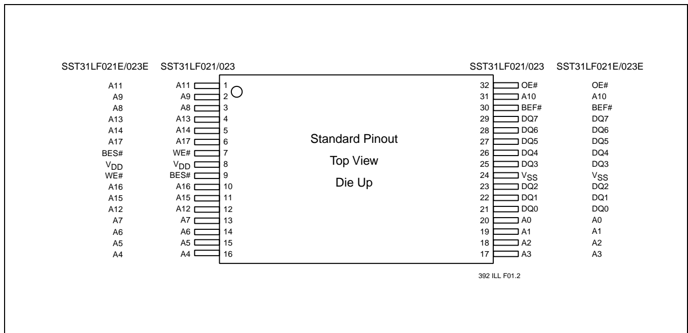
FIGURE 1: PIN ASSIGNMENTS FOR 32-PIN TSOP (8MM X 14MM)
