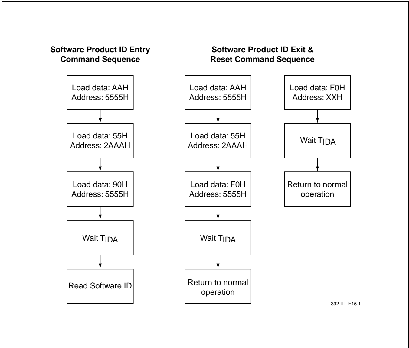
FIGURE 18: SOFTWARE PRODUCT COMMAND FLOWCHARTS
