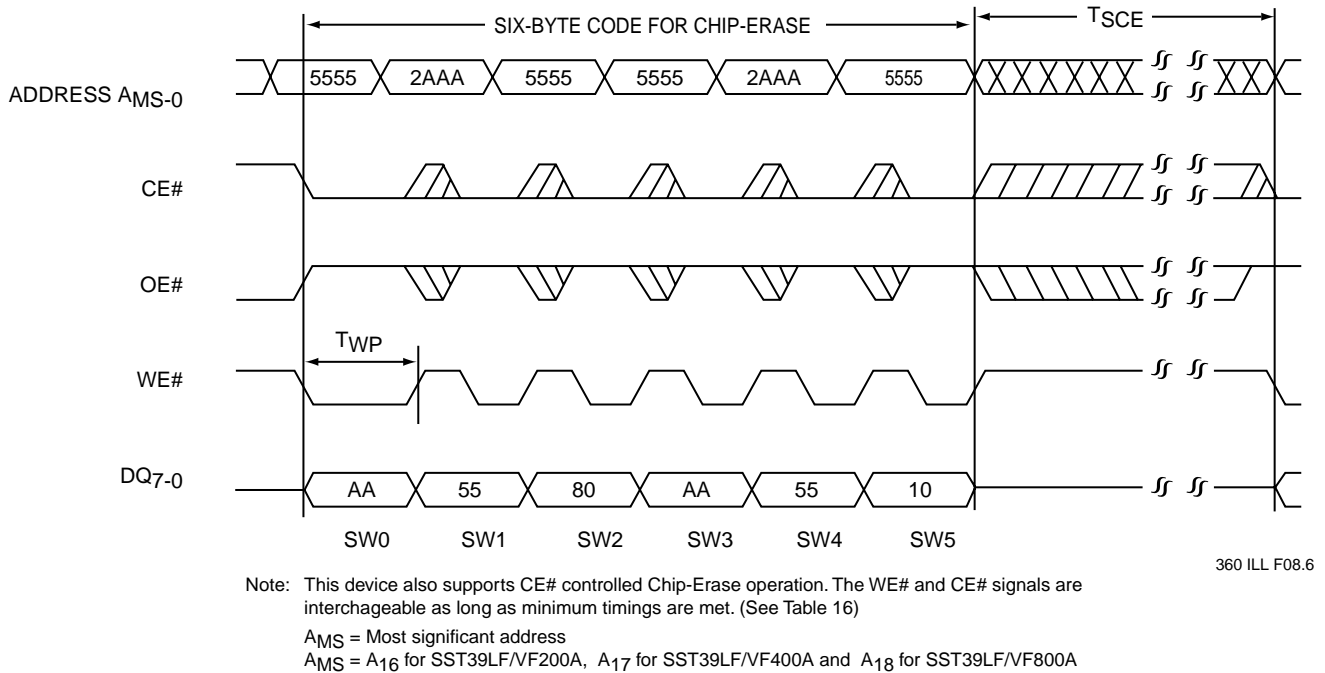
FIGURE 8: WE# CONTROLLED CHIP-ERASE TIMING DIAGRAM
