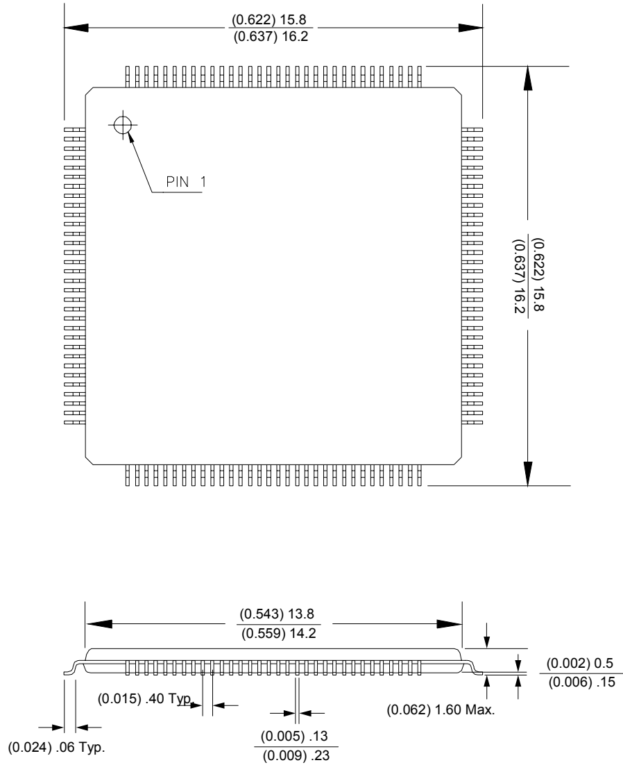
78P2352-IGT 128-pin Standard JEDEC LQFP (Top View)
